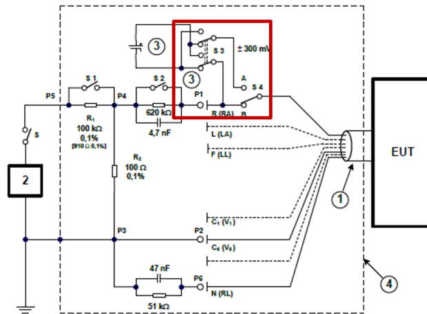
Figure 101: AECG100 \pm 300\text{mV} DC offset
