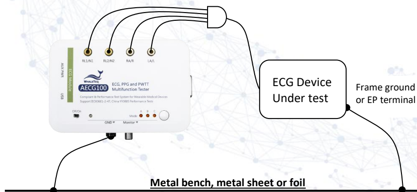
Figure 8: ECG Test Mode with Noise Reduction Product Wiring Diagram
