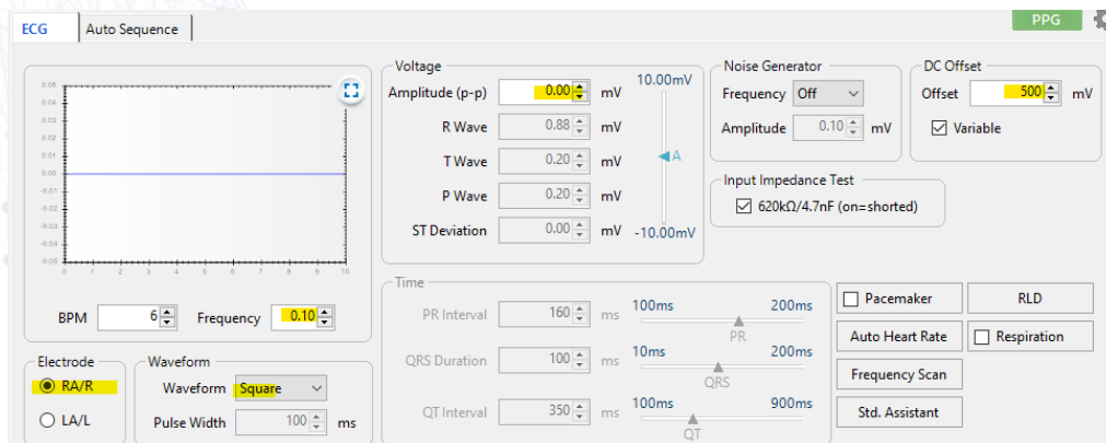
Figure 104: DC Voltage Verification (&gt;300mV)
